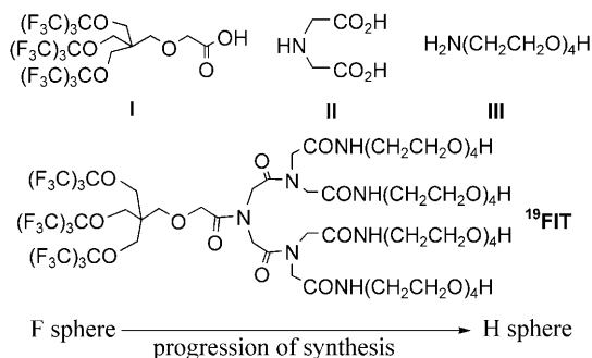
Figure 1. Chemical structures of ^{19}\text{F} IT and its three building blocks (I, II, and III). ^{19}\text{F} IT is designed to be a bispherical cone. The F sphere contains 27 fluorine atoms for ^{19}\text{F} signal generation. The H sphere, currently made of 4 OH groups, can be derivatized to COOH, \text{NH}_2 , and SH for future drug conjugation. [23]
