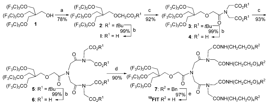
Scheme 1. The synthesis of ^{19}\text{F} IT. Reaction conditions: a) KH, \text{BrCH}_2\text{CO}_2t\text{Bu} , THF, RT, 12 h; b) TFA, anisole, \text{CH}_2\text{Cl}_2 , RT, 2 h; c) DIC, HOBT, DMF/THF (1:1), \text{HN}(\text{CH}_2\text{CO}_2t\text{Bu})_2 (=II-( t\text{Bu} ) 2 ), RT, 12 h; d) DIC, HOBT, DMF/THF (1:1), \text{H}_2\text{N}(\text{CH}_2\text{CH}_2\text{O})_4\text{Bn} (=III-Bn), RT, 18 h; e) \text{H}_2 , Pd/C, MeOH, RT, 12 h. TFA = trifluoroacetic acid, DIC = 1,3-diisopropylcarbodiimide, HOBT = 1-hydroxytriazole, DMF = N,N' -dimethylformamide, THF = tetrahydrofuran Bn = benzyl.
